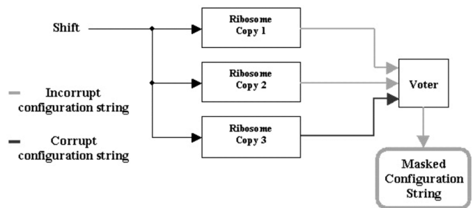
Fig. 15. Triple modular redundancy masking of a gene fault.
