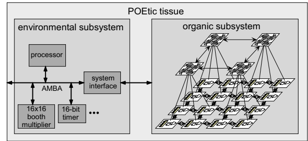
Figure 1. The POEtic chip, showing the microprocessor and the reconfigurable array. In the organic subsystem, the molecular plane (bottom) is connected to the routing plane (top). Many elements connected to the AMBA bus, (another timer and serial and parallel ports) are omitted in order to simplify the schematics.
